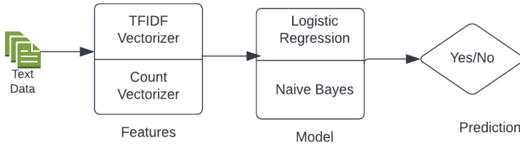
Fig. 5. Design of Text Classification Model
