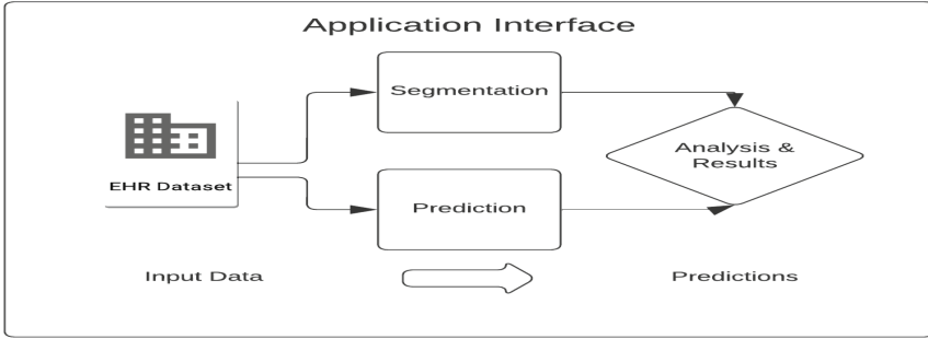
Fig. 1. Application Interface
