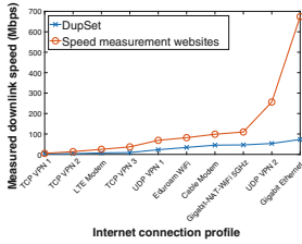
Fig. 5. Correlation between traditional Internet speed measurement (average result from nine websites) and DUPSET probes over 10 different Internet connection profiles.
