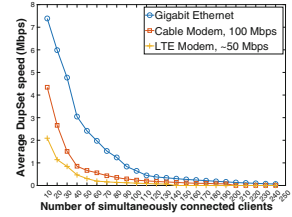
Fig. 7. Average DUPSET readings for different types of Internet connection profiles with different number of clients simultaneously served by a SMARTWiFi router.
