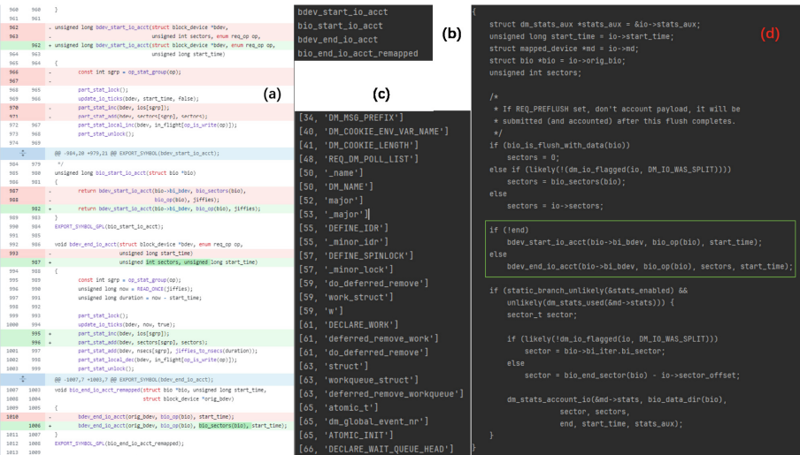
Fig. 2. A demo of our toolkit. (a) A code diff as described below. (b) The list of identifiers that being modified. (c) Part of identifier list derived from preorder traversal of AST. (d) The result we get after the relevant part edited by GPT-4.
