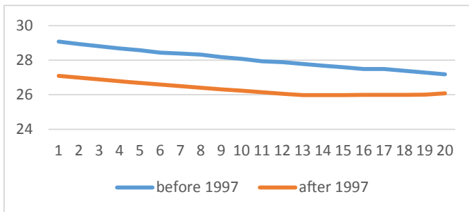
Fig. 4. The change rate of forest area
