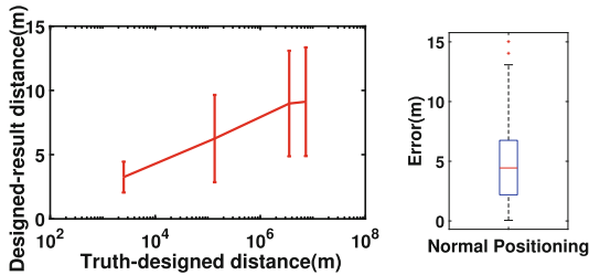
Fig. 7. Static external signal attack evaluation
