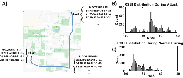
Fig. 8. Dynamic attack route and RSSI distribution
