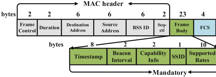
Fig. 3. The structure of spoofing beacon frame packet.
