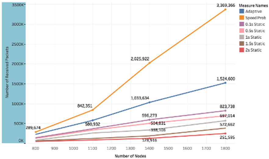
Fig. 3. Received packets
