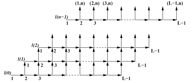
Figure 1: Directed graph for the computation of c^n(i, j) .
