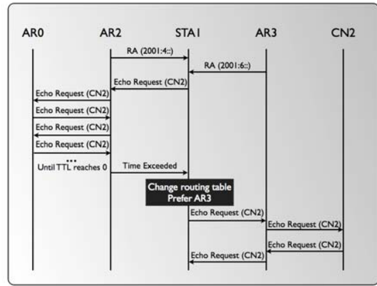
Figure 6: Message flows for Scenario 3
