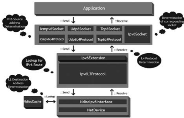
Figure 2: The IPv6 implementation overview
