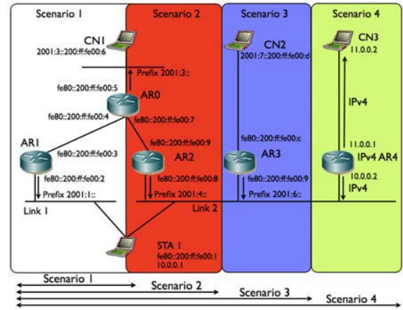
Figure 3: Topology of the first 4 trials
