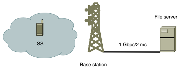
Figure 3: Network structure.
