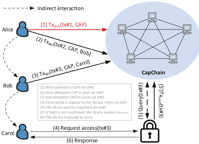
Fig. 4. CapChain overview [20].
