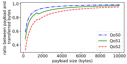
Fig. 5. Ratio between payload and transmitted bytes for different MQTT QoS levels.
