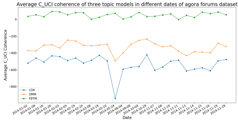
Fig. 4. Average UCI coherence of three topic models in different dates of Agora forums
