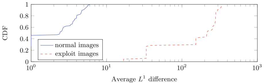
Fig. 4. Cumulative distribution function (CDF) of the average L^1 distance (Eq. 1) between the output of two decoders on the same input JPEG image. The CDF of the normal images is cleanly separable from that of the exploit images.
