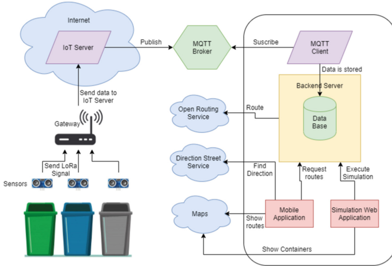
Fig. 1. General configuration and communication of system components
