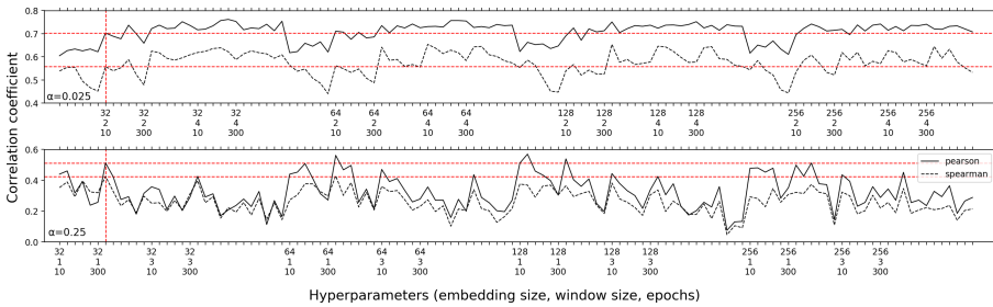
Fig. 2. Correlation values between calculated relatedness scores and cosine similarities, across all pairs of file hashes, for a range of hyperparameter values.
