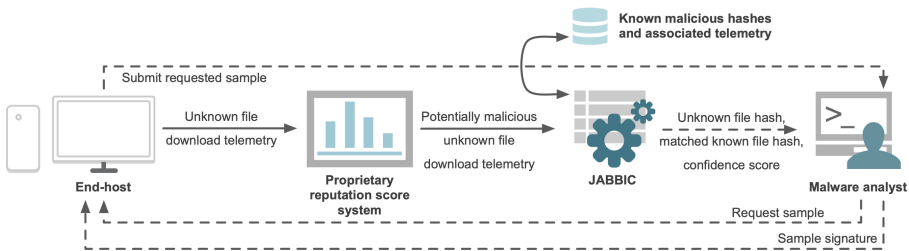
Fig. 1. Improved triage of unknown files using JABBIC at the interface between proprietary reputation score systems and malware analysts.
