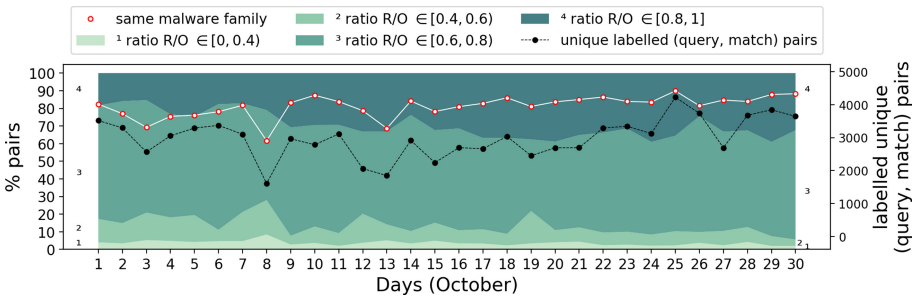
Fig. 4. Percentage of query file hashes and their match file hashes from each previous day of October 2015 with the same malware families. The plot also shows the proportion of pairs falling into each R/O band.
