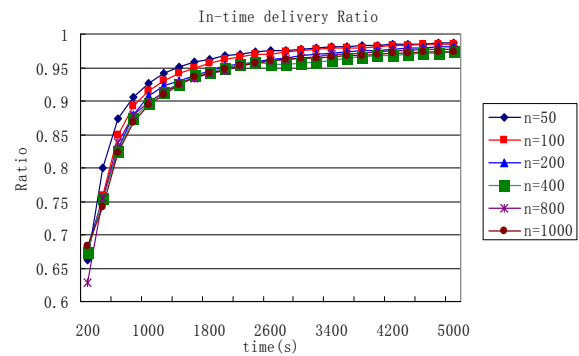
Figure 8. In-time delivery ratio as a function of time under different swarming scales
