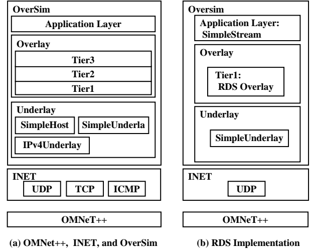
Figure 5. Simulation framework and prototype implementation
