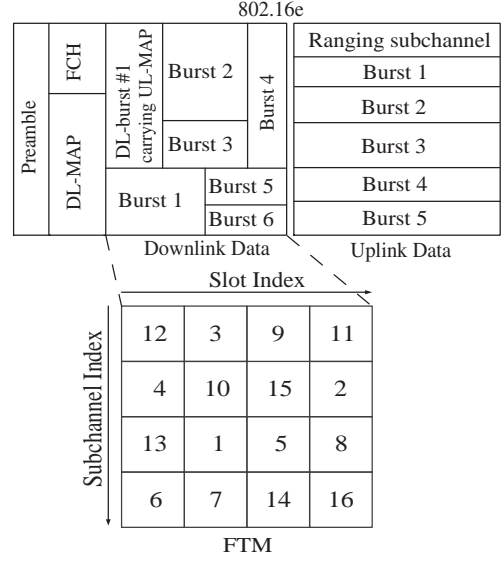
Figure 3: An example of time slot rearrangement by FTM.
