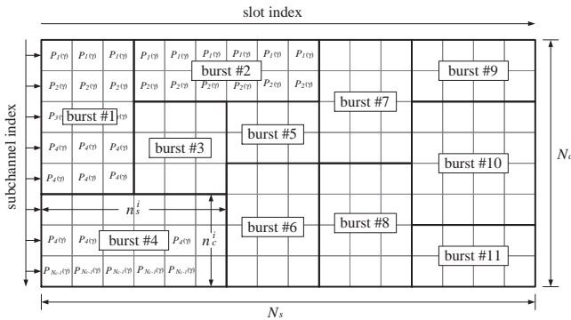
Figure 1: The diagram of the frame structure of IEEE 802.16e.
