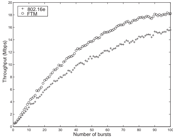
Figure 7: The comparison of throughput of IEEE 802.16e and FTM vs. N_B with \gamma_n = 64\text{-QAM } 3/4 and P_i(\gamma) \in [0.5, 1] .
