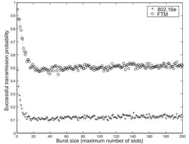
Figure 6: The successful transmission probability vs. M (maximum number of slots).
