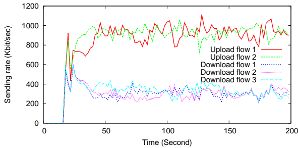
Figure 8: TFRC sending rate
