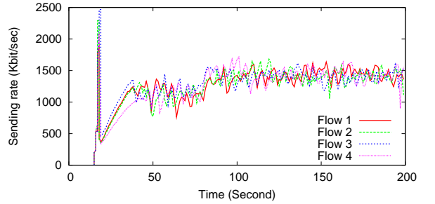
Figure 5: TFRC sending rate
