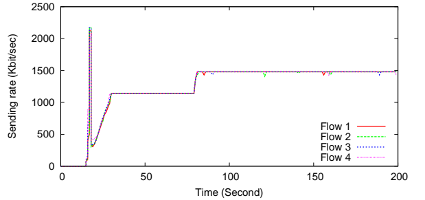
Figure 6: MTFRC sending rate
