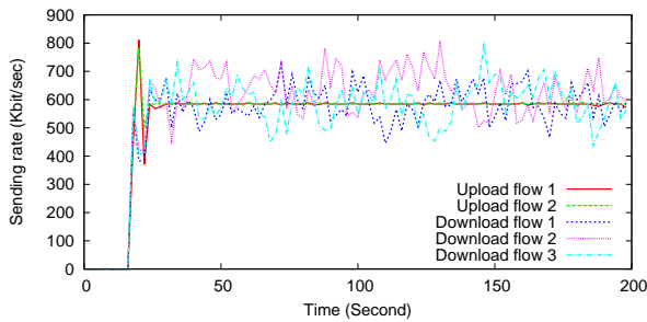
Figure 9: Sending rate with MTFRC
