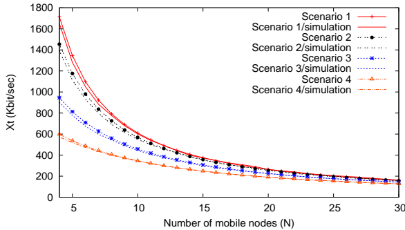
Figure 2: Evolution of X_t in UDP mode as a function of the number of uploading mobile nodes
