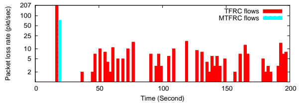
Figure 7: Packet loss rate of TFRC and MTFRC aggregates
