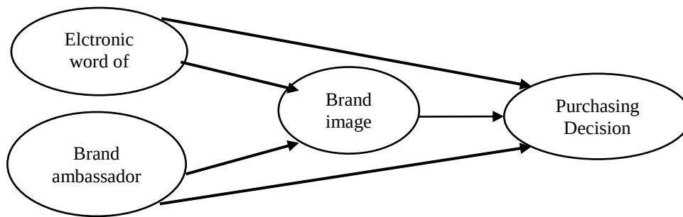
Fig. 1. Conceptual Framework
