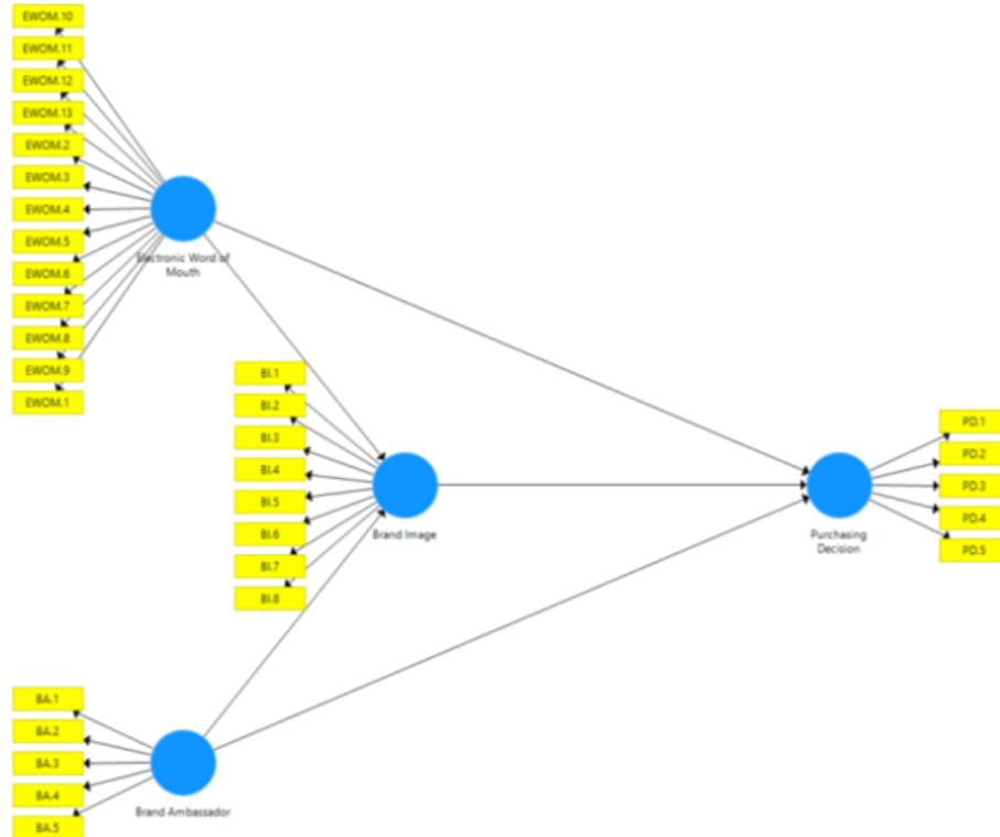
Fig. 2. SEM-PLS Model
