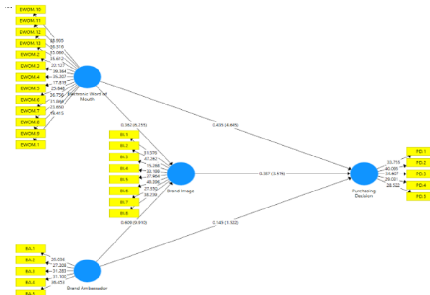
Fig. 2. SEM-PLS Algorithm
