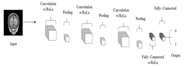
Fig 6: Architecture of DCNN (Proposed)
