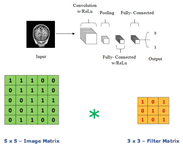
Fig 2: CNN architecture with 4 layers (Proposed)
