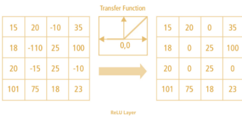
Fig 4: ReLU operation
