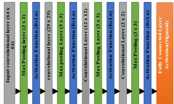
Fig 7: Architecture of DCNN System (Proposed)
