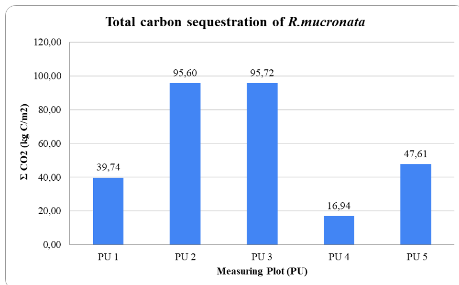
Fig. 3. Total carbon storage of Rhizophora mucronata in Baros mangrove conservation forest.
