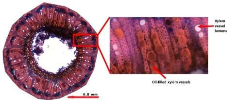
Fig.5. Presence of oil in the xylem vessels. Cross-sectional view of the stem of A. alba .
