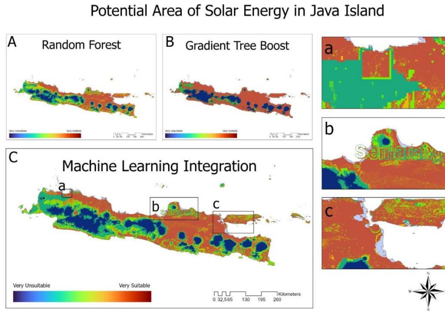
Fig. 3. Potential area of solar energy in Java Island with machine learning algorithms, such as: Random Forest (A), Gradient Tree Boost (B), and machine learning integration (C) in the DKI Jakarta (a), Semarang (b), and Surabaya (c).
