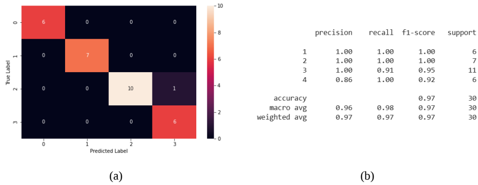
Fig. 2. (a) Confusion Matrix (b) Confusion matrix evaluation
