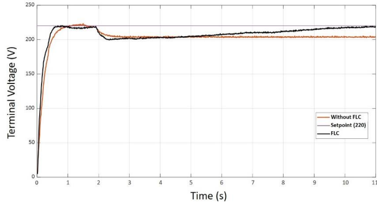
Fig. 8. AVR with resistive load.
