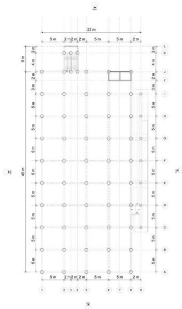
Fig. 13. Building Plan
