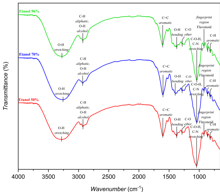
Fig. 1. FTIR spectrum of soursop peel extract.
