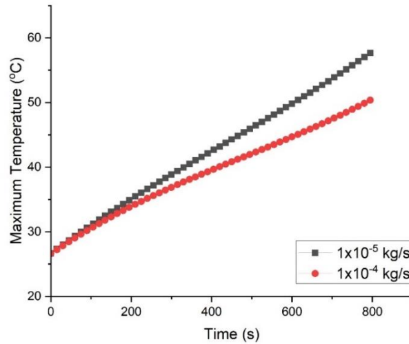
Fig. 7. Maximum temperature of lithium-ion battery with 50% ethylene glycol cooling fluid at different mass flow rate
