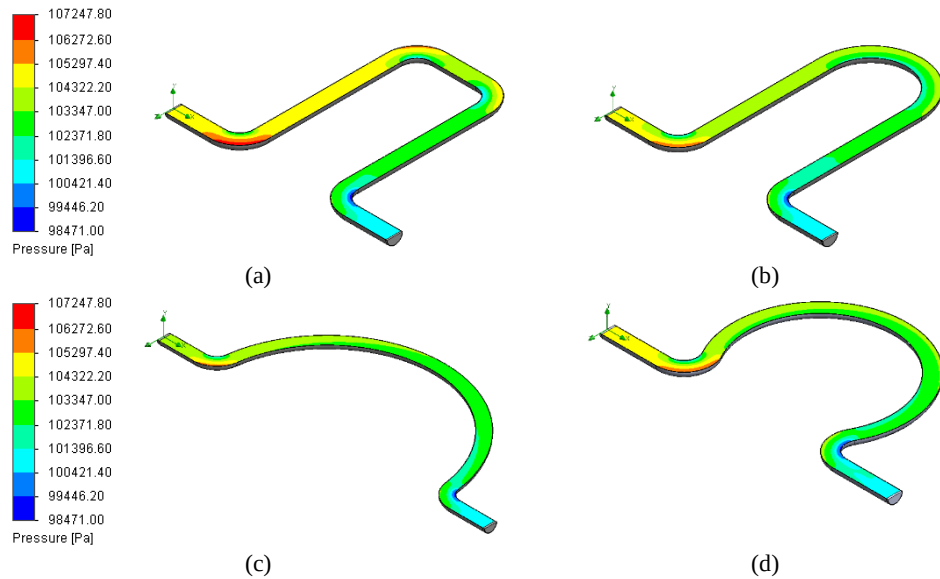
Fig. 7. Pressure contour on (a) type I, (b) type II, (c) type III, and (d) type IV in the simulation with a fluid density of 950 kg/m 3 .
