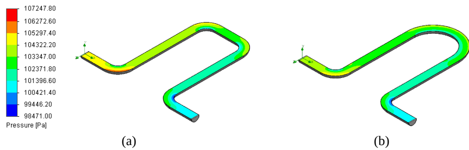
Fig. 7. Pressure contour on (a) type I, (b) type II, (c) type III, and (d) type IV in the simulation with a fluid density of 950 kg/m 3 .
