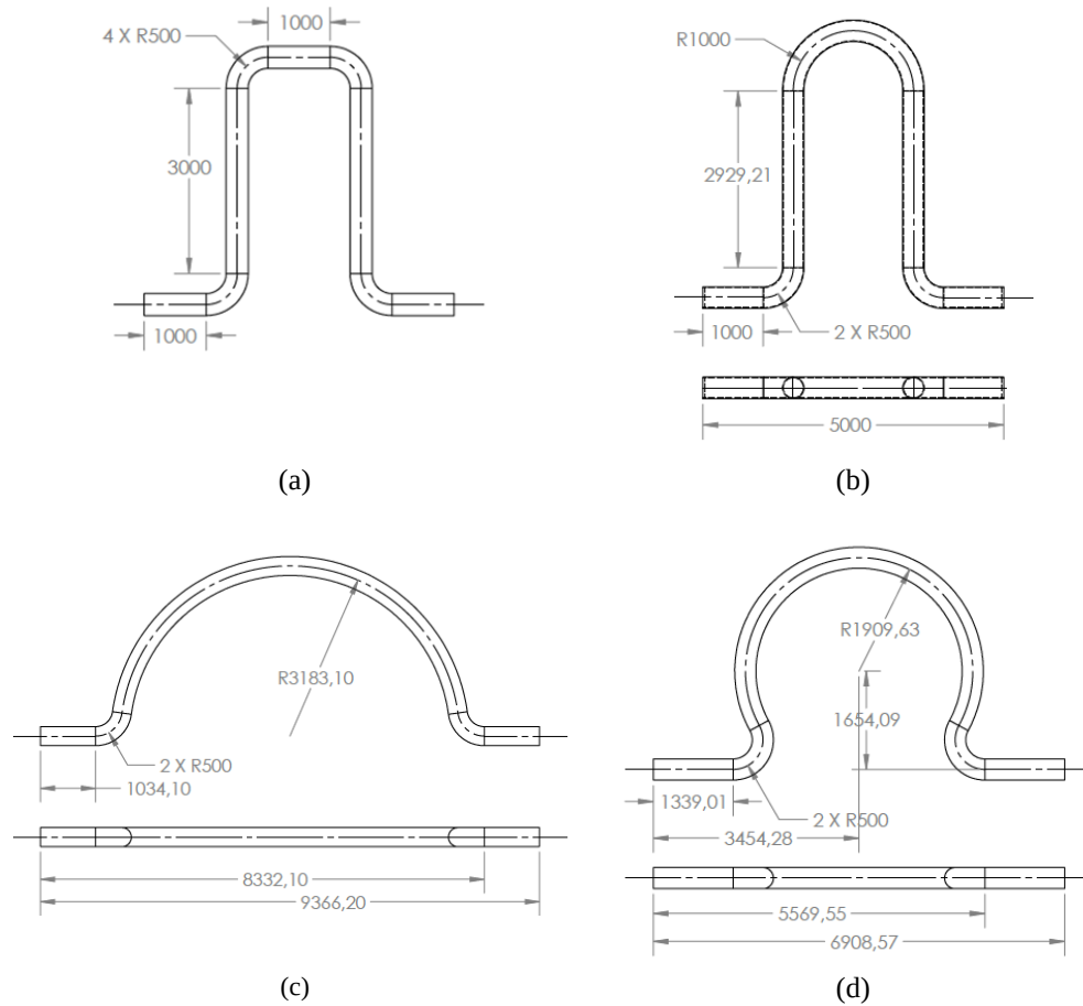
Fig. 2. Expansion loop design that has been made, (a) type I, (b) type II, (c) type II and (d) type IV in millimeters (mm).
