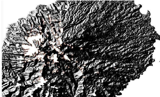
Fig. 12. Hill shade analysis of Manali Hills
