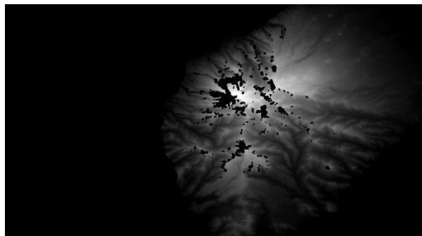
Fig. 13. Ruggedness Index analysis of Manali Hills
