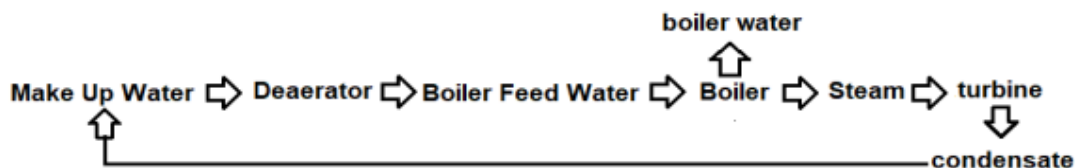
Fig. 1. Flow of Boiler Water System
