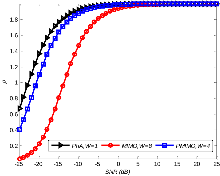
Fig. 1. SNR detection performance of various types of radar.
