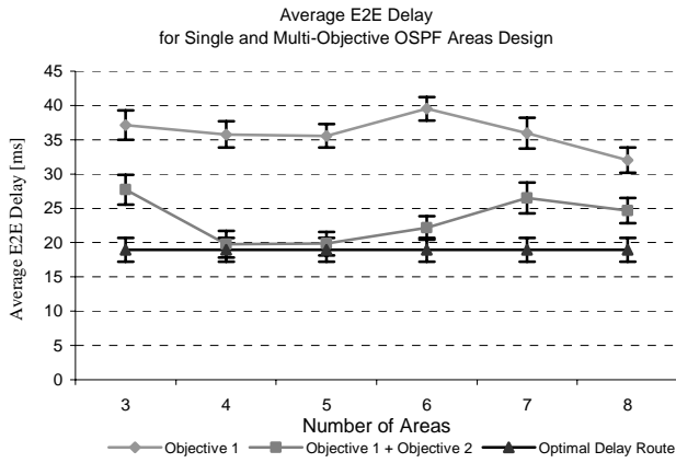
Figure 4. Multi-objective optimization effect on end-to-end delay performance
