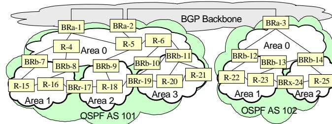
Figure 2. Division of 25 OSPF routing into a routing hierarchy, where most LSAs are broadcast only within their small OSPF areas.
