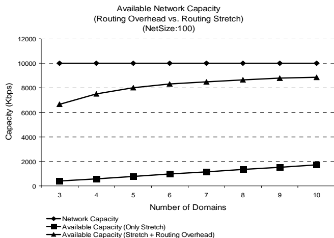
Figure 5. Multi-objective optimization effect on available network capacity
