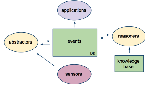
Fig. 1. Context determination using abstraction and reasoning.
