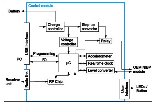
Figure 2. Description of the system's parts and interfaces.
