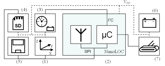
Figure 1. Hardware architecture of the Motionlogger.
