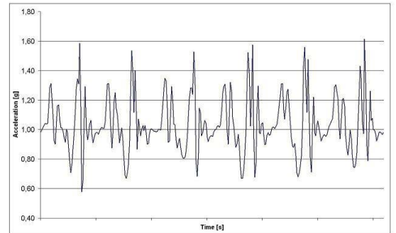
Figure 3. Resulting acceleration pattern for walking. (Independent of the Motionlogger's orientation)
