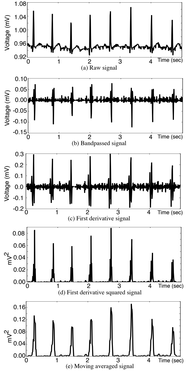
Fig. 5: RR interval feature extraction process. (a) shows the initial raw ECG signal. (b)-(e) illustrate the result of each processing step.
