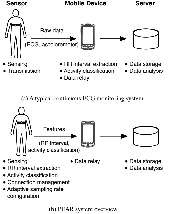
Fig. 1: A comparison of typical framework of continuous ECG monitoring system (a) and PEAR system overview (b).
