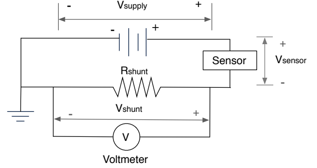
Fig. 6: Shunt circuit used for energy profiling.
