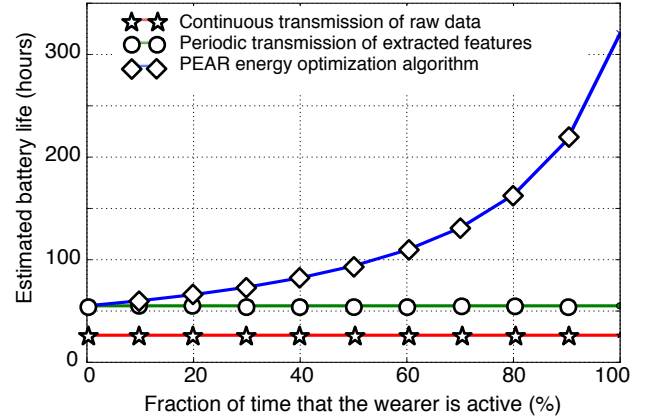
Fig. 8: Sensitivity analysis showing the estimated battery life for a SHIMMER sensor node (280mAh battery capacity), based on the fraction of time that wearers are active. In a small user study, participants were active 20.4% of the time on average.
