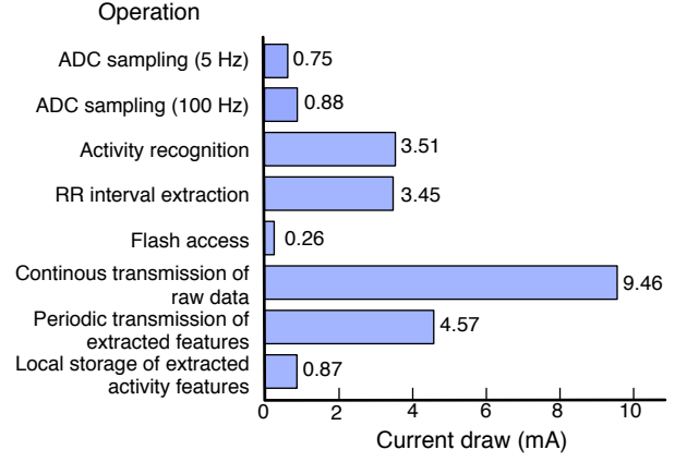
Fig. 7: Current draw characteristics for each operation.
