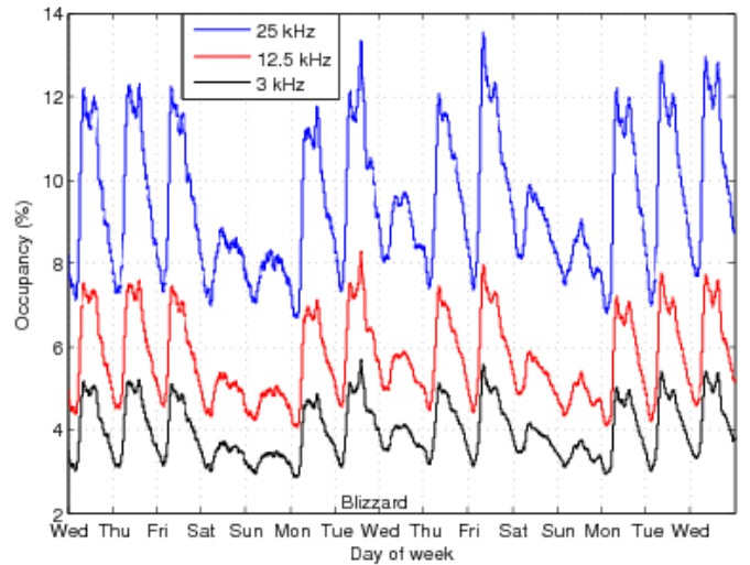
Figure 1. Occupancy vs. time for fifteen day period in 2011 for 3, 12.5 and 25 kHz bandwidths
