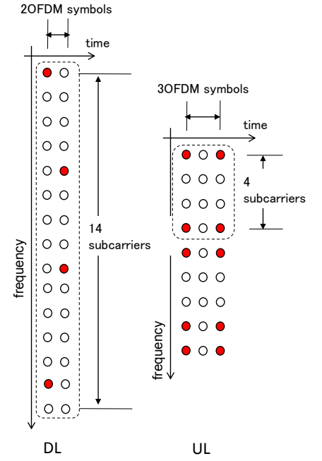
Fig. 5 Pilot symbol assignment for mode 1 (FFT size: 1024).
