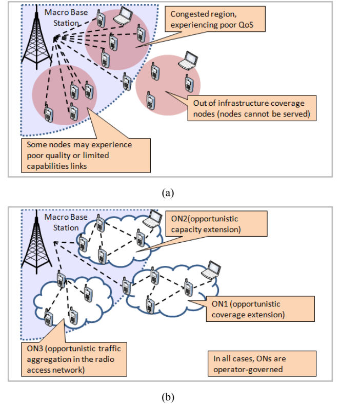
Figure 1. (a) Various problematic situations which may occur to a network, without the use of opportunistic networks, (b) Solutions to network issues by incorporating the indicative business scenarios of the opportunistic networks
