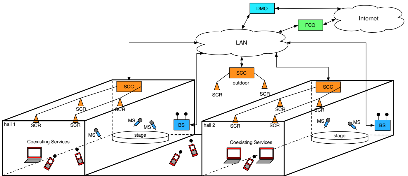
Fig. 1: General overview of the field trial platform
