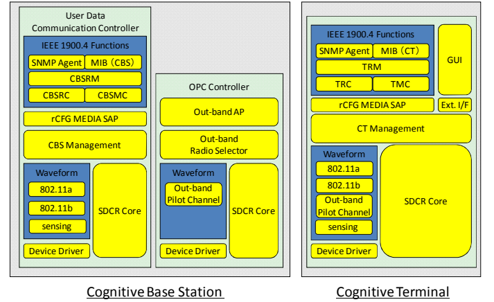
Figure 5. Software architecture of CBS (left) and CT (right)
