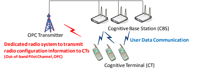
Figure 2. Out-of-band Pilot Channel for spectrum sharing type CRS
