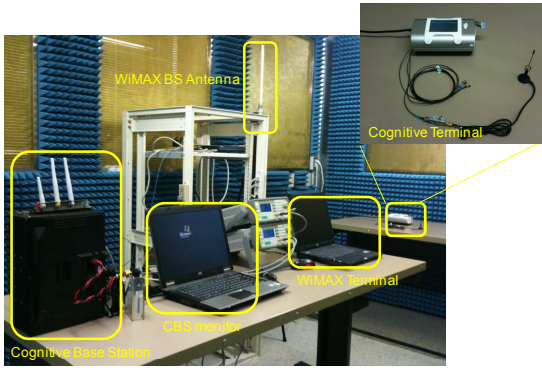
Figure 6. Evaluation environment in shield room
