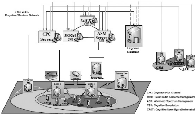
Fig. 2. Architecture of the CRS testbed
