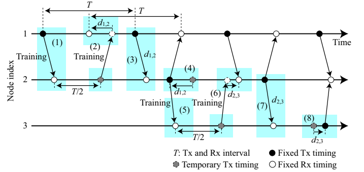
Fig. 7. Procedure of network synchronization scheme.
