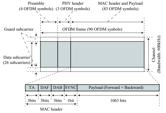
Fig. 6. Frame configuration.
