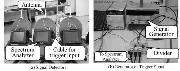
Fig. 5. Equipments of Constructed Measurement System
