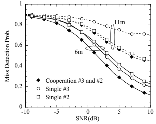
Fig. 8. Performance between Miss Detection Prob. and SNR
