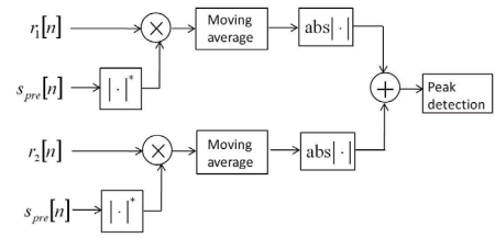
Fig. 5. Synchronization Scheme 1.
