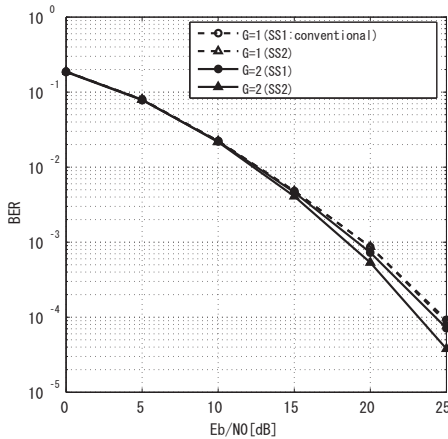
Fig. 9. BER performance in the NLOS condition (threshold level=0.6).
