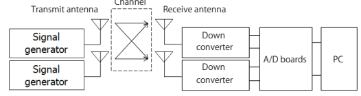
Fig. 2. Experiment system.
