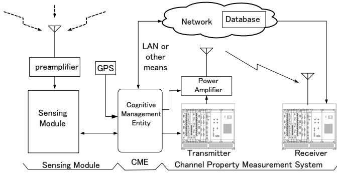
Fig. 1. NICT TVWS prototype block diagram.
