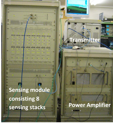
Fig. 2. The NICT TVWS prototype hardware showing the sensing module consisting of 8 sensing stacks and transmitter.
