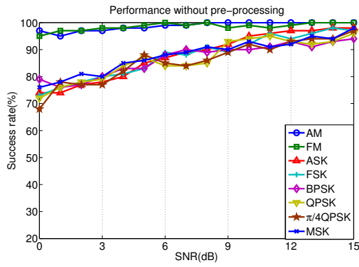
Fig. 5. Classification performance without pre-processing
