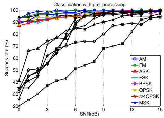
Fig. 6. Classification performance with pre-processing (color) and performance compared with [4] (black)
