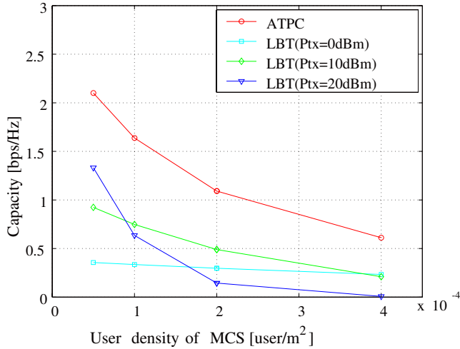
Fig. 9. Area-averaged cell capacities achieved by the CRS versus the effective user density of the MCS MS, outdoor
