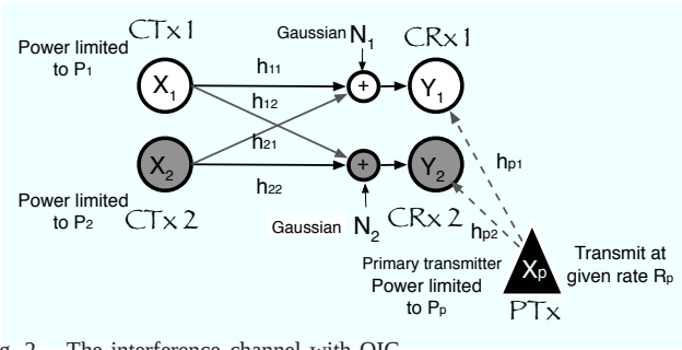
Fig. 2. The interference channel with OIC.
